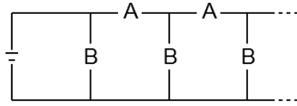
FIG. 7.1. An electric circuit whose joint resistance is related to the matrix geometric mean
