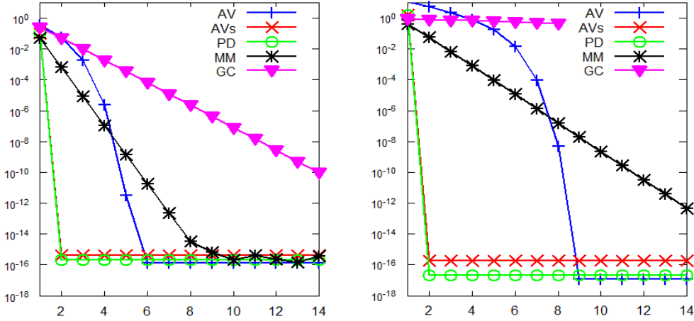
FIG. 8.1. Comparison of the accuracy obtained at various steps by the Averaging iterations (AV), by the Averaging iteration with spectral scaling (AVs), by the polar decomposition algorithm (PD) and the accuracy for various number of nodes of the rational minimax approximation algorithm (MM) and of the Gauss-Chebyshev quadrature (GC) on Test 8.1 for x = 10 (left) and x = 1000 (right).
