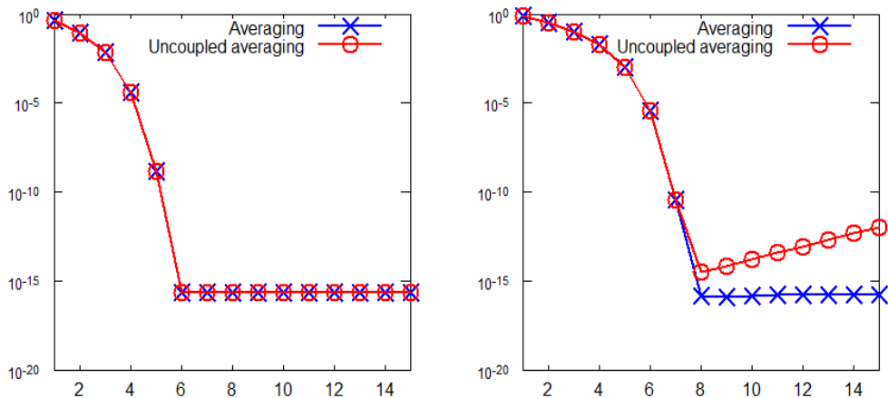
FIG. 8.3. Iteration step vs. relative error for the averaging iteration and its uncoupled version for t = 0.5 (left) and t = 1.5 (right) as in Test 8.3. In the second case the derivative of G(X) has spectral radius greater than one and the uncoupled iteration shows numerical instability.
